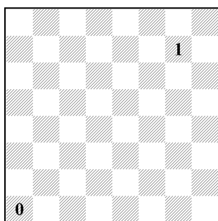
Leaper [ 6 , 6 ]
