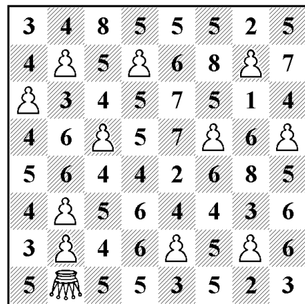
11 pawns / 52 squares
