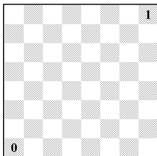
Leaper [ 7 , 7 ]
