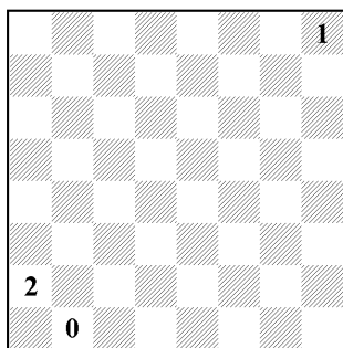
Leaper [ 6 , 7 ]
